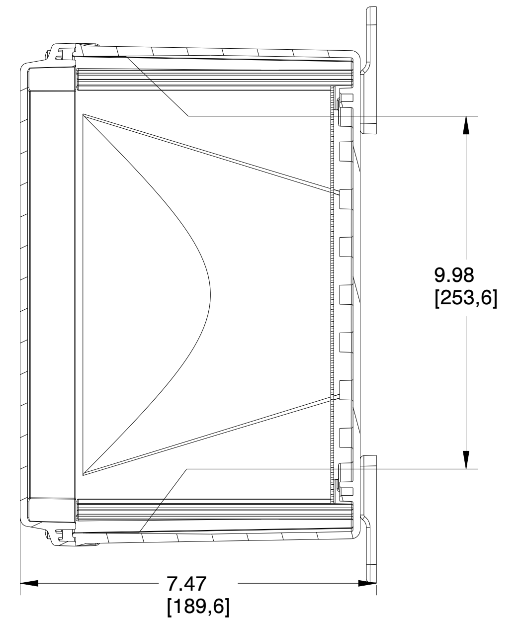
SECTION B-B
