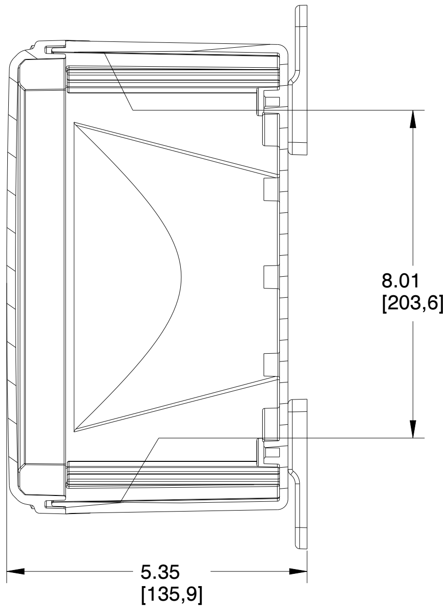
SECTION B-B
