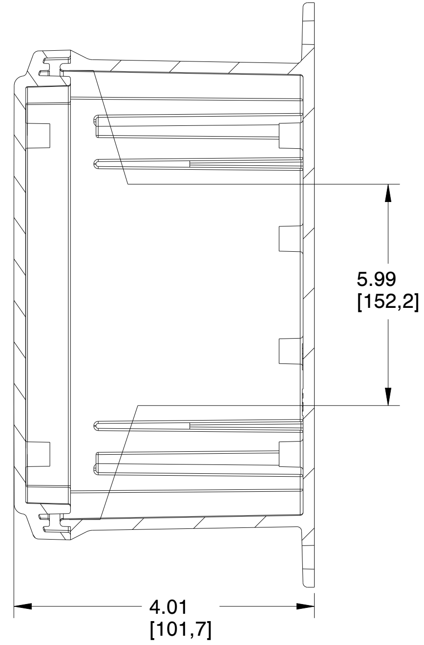
SECTION B-B
